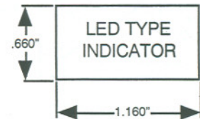
PANEL CUT-OUT RP3 LED INDICATOR NOTE: DRAWING NOT TO SCALE.
