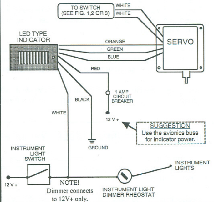
FIGURE 4 LED TYPE POSITION INDICATOR
