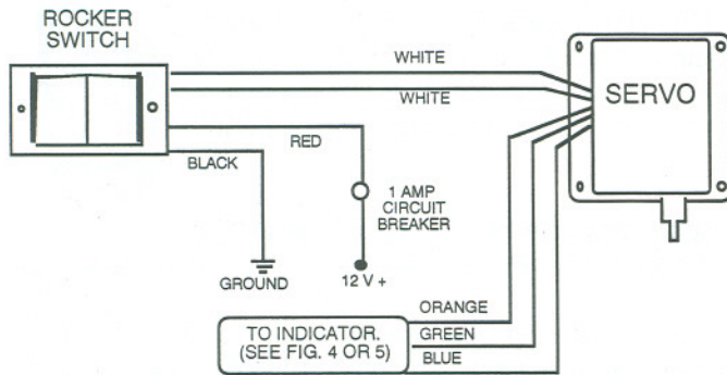
FIGURE 3 DPDT SWITCH
