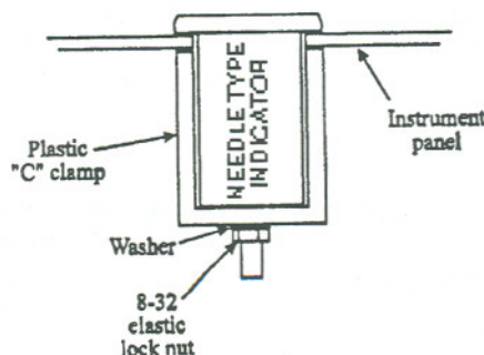
PANEL CUT-OUT RP2 NEEDLE INDICATOR NOTE: DRAWING NOT TO SCALE.
