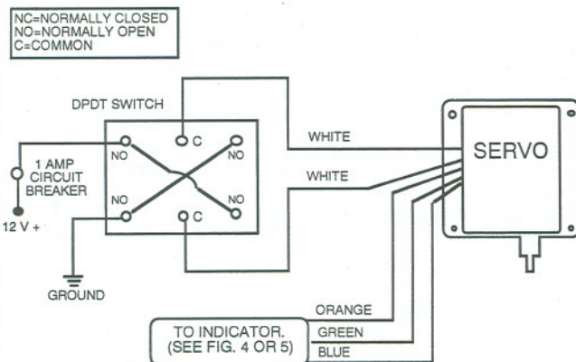
FIGURE 3 DPDT SWITCH
