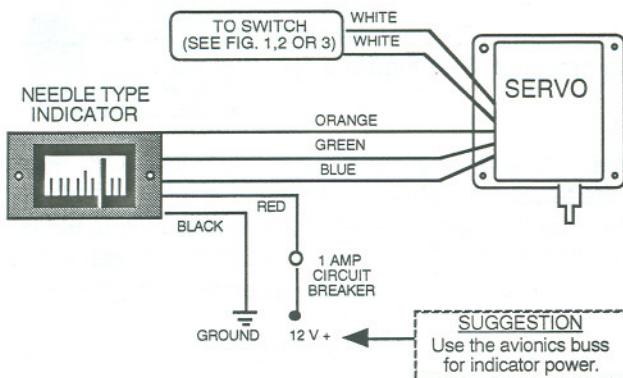
FIGURE 5 NEEDLE TYPE POSITION INDICATOR
