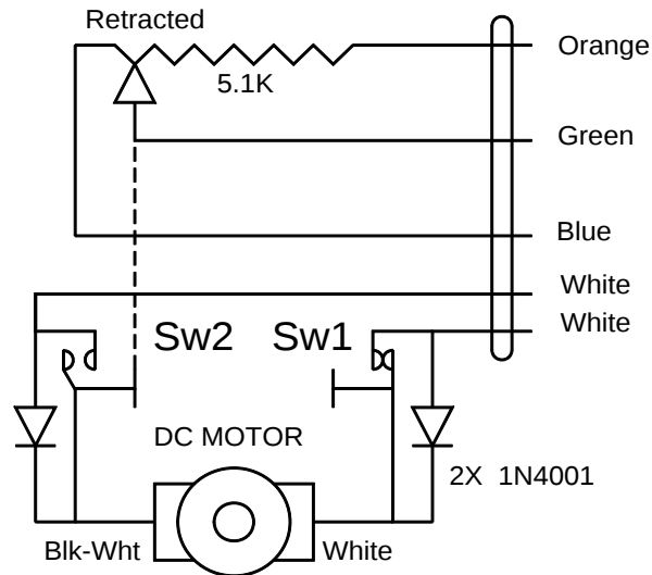
MAC8A Schematic
